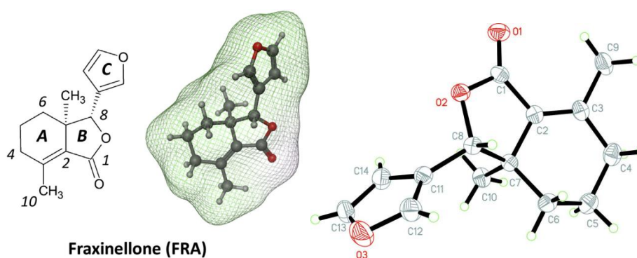
Fig. 1. Structure of fraxinellone
