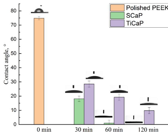
Fig. 2. Contact angle of water on polished PEEK, SCaP and TiCaP coatings
