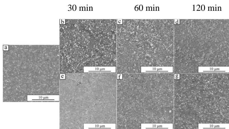
Fig. 1. SEM images of, (a) polished PEEK, (b-d) SCaP and (e-g) TiCaP coatings
